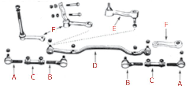
A: Outer Tie Rod Ends B: Inner Tie Rod Ends C: Tie Rod Adjusting Sleeves D: Center Link E: Idler Arm F: Pitman Arm
